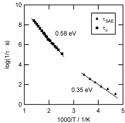
Fig. 2: 1/\tau_{\text{SAE}} and 1/\tau_{\sigma} as a function of the inverse temperature. Whereas 1/\tau_{\sigma} probes Li transport on a long-range length scale, 1/\tau_{\text{SAE}} is additionally sensitive to spatially confined \text{Li}^+ motions.
