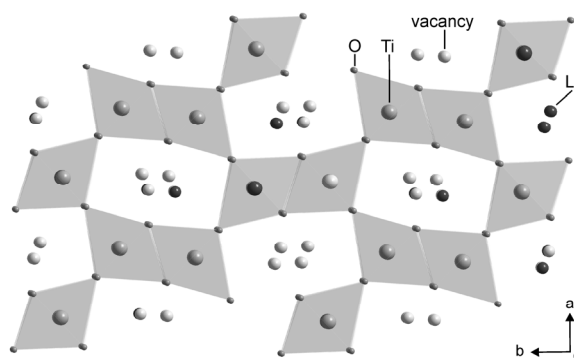
Fig. 1: Crystal structure of \text{Li}_2\text{Ti}_3\text{O}_7 .
