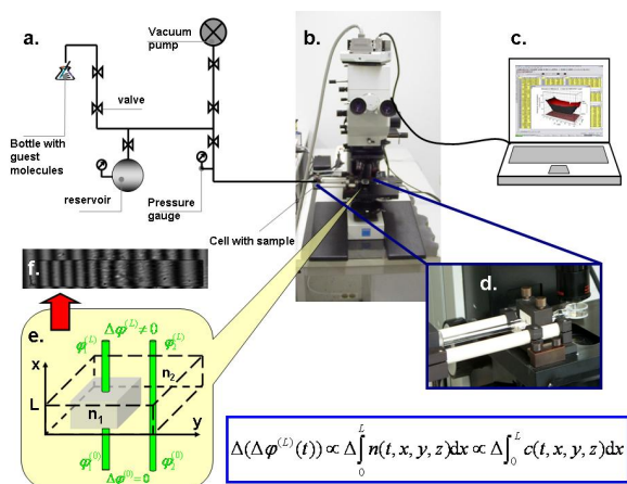
Figure 1: Schematics of diffusion measurement by interference microscopy (DIF) a. Schematic drawing of the vacuum system; b. Interference microscope and the cell with the sample placed underneath its lenses; c. Computer connected to the camera for further analysis of the data; d. The cell with the sample under magnification; e. Schematic drawing of the principle; f. Interference pattern of an investigated crystal; The mathematical relation on the bottom side of the figure shows the proportionality between the change of intracrystalline concentration and of phase-difference between the light beams.
