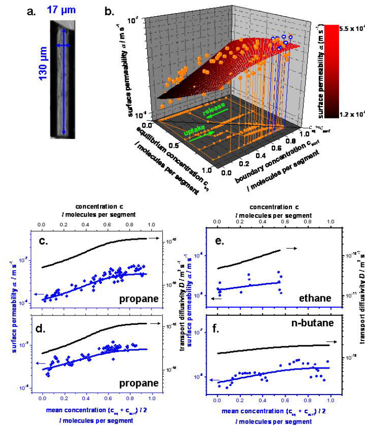
Figure 2: a. The crystal under study; b. Surface permeability as a function of the boundary and equilibrium concentration of propane; c. –f. Concentration dependencies of transport diffusivities and surface permeabilities ( d. refers to another specimen of the sample).
