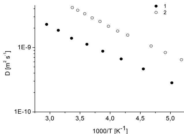
Fig. 1: Temperature dependence of effective diffusion coefficient 1 – diffusion coefficient in glass bed of sample 3; 2 – diffusion coefficient of pure liquid n-hexane
