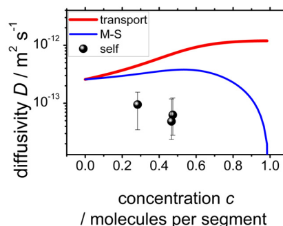
Figure 1: Maxwell-Stefan (M-S), transport and self-diffusivity of propane in MOF Zn(tbip), taken from ref. [1].
