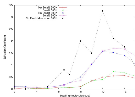
Fig. 2: The variation of the self-diffusion coefficient D , in units of 10^{-10} \text{ m}^2\text{s}^{-1} , with concentration at T = 500 \text{ K} and 600 \text{ K} .
