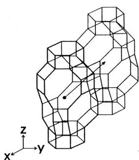
Fig. 1: Schematic view of the chabazite framework.
