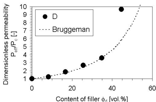
Fig. 1: The comparison of experimental P_{eff}/P_c vs. \phi_d plot for membrane made of PI(6FDA-ODA) with theoretical dependence simulated using the model by Bruggeman.
