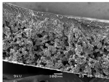
Fig. 2: The SEM image of membrane made of PI(6FDA-ODA) filled by 60 wt. % of silicalite-1.
