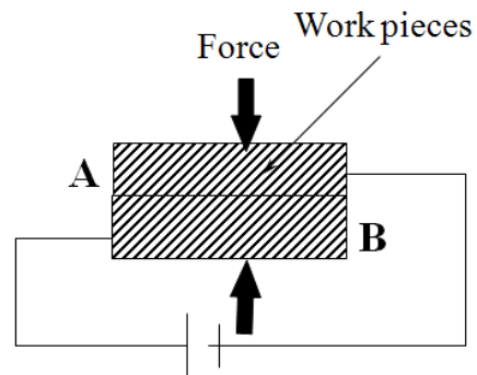
Figure - Schematic representation of diffusion welding using electrical resistance for heating
