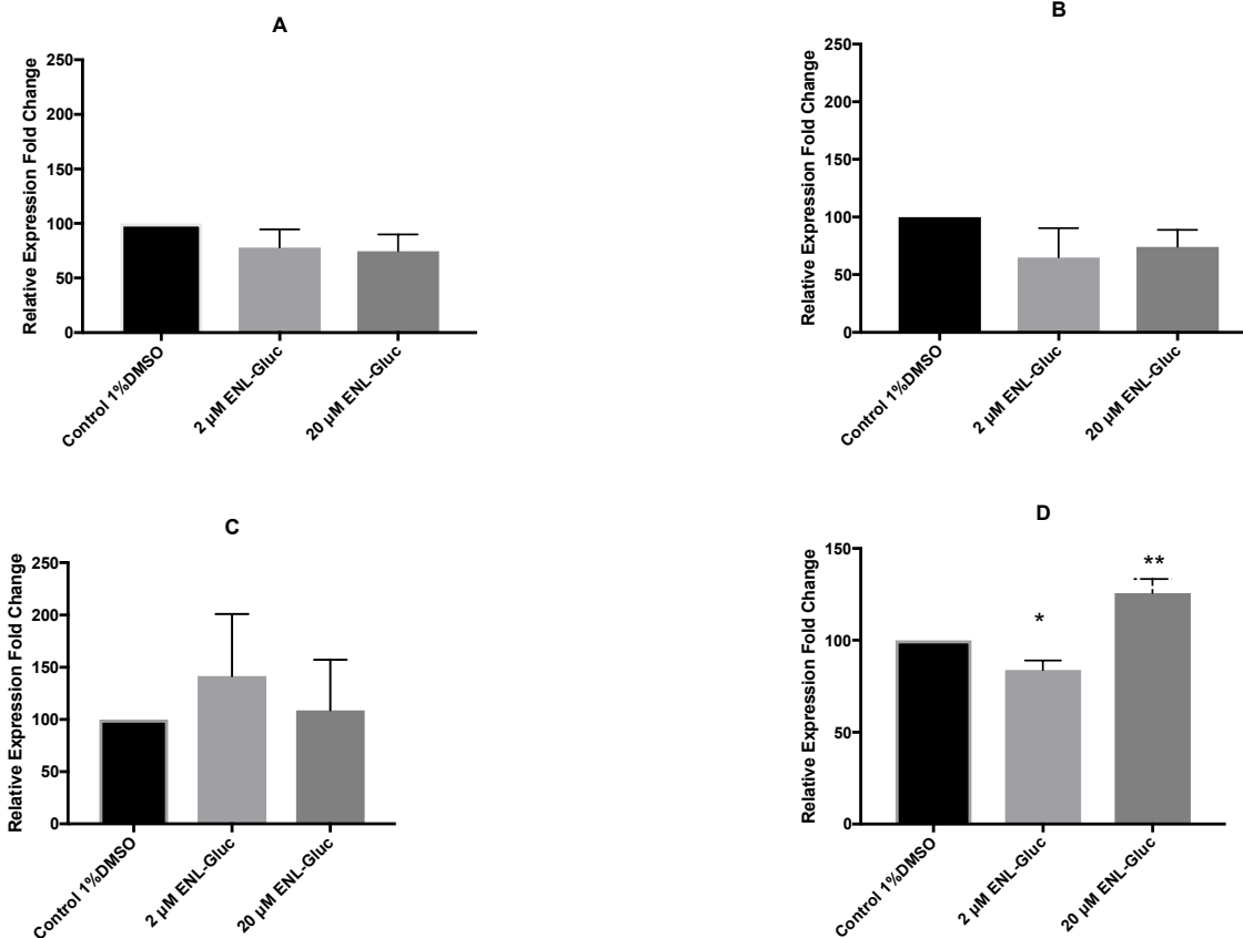
Figure 7.10. Effect of enterolactone glucuronide (ENL-Gluc) on the protein level of A) HMGCoA-AR, B) LDL-R, C) INSIG-1 and D) SREBP-2 in HepaRG cell line treated with 2 and 20 μM of ENL in the absence of U18666A for 24 hours. Data is presented in percent as mean ± S.D, n=3 (3 technical replicates and on three separate occasions), * p-value < 0.05, ** p-value < 0.01.
