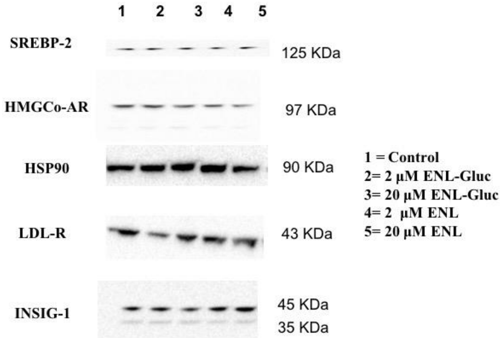
Figure 7.9. Effect of enterolactone (ENL) and/or enterolactone glucuronide (ENL-Gluc) on HMGC o A-R, INSIG-1, and SREBP-2 protein level. ENL decreased the protein level of HMGC o A-R while increasing the protein level of LDL-R and INSIG-1 and SREBP-2. ENL-Gluc decreased the protein level of HMGC o A-R and LDL-R and at higher concentration increases INSIG-1 level with no noticeable influence on SREBP-2 protein expression following western blot assay. Representative pictures of (n = 3).
