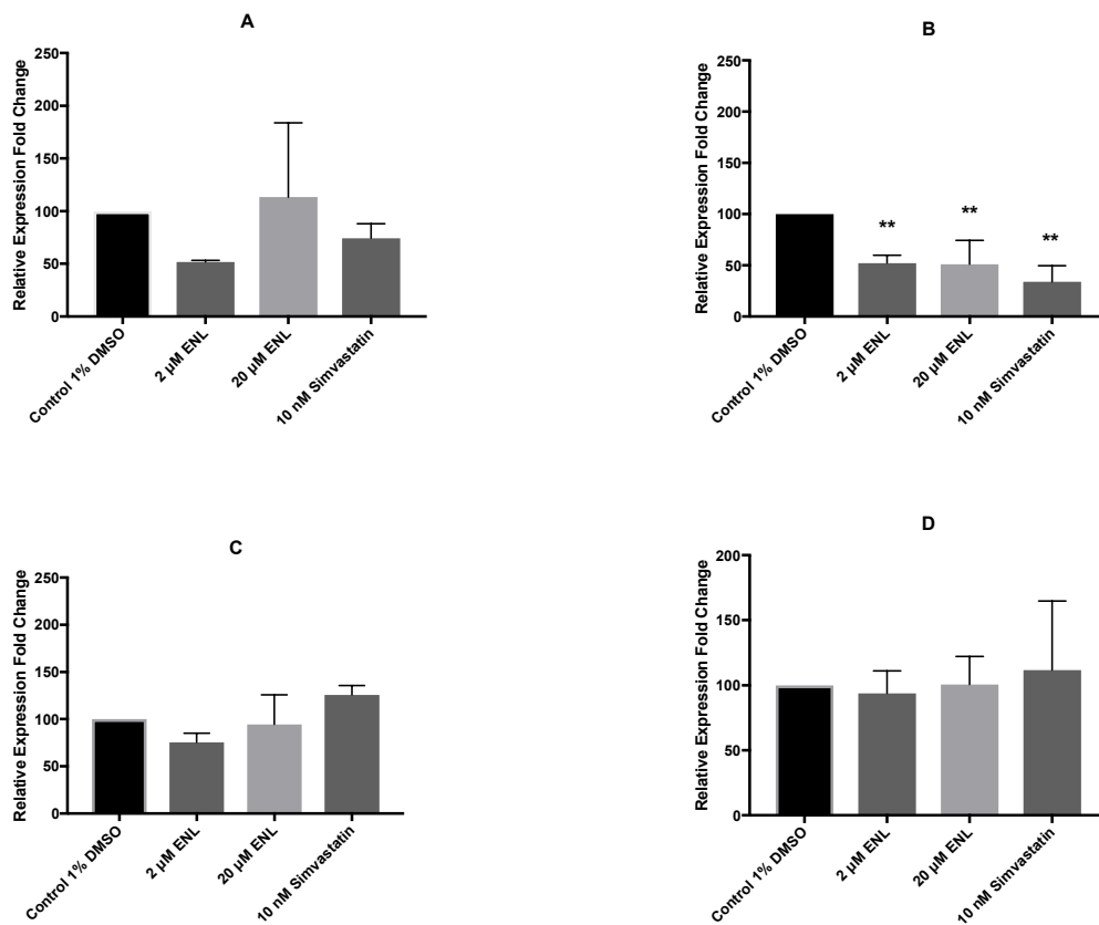
Figure 7.8. Effect of enterolactone (ENL) on the relative mRNA expression of A) HMGCoA-AR, B) LDL-R, C) INSIG-1 and D) SREBP-2 in HepaRG cell line treated with 2 and 20 μM of ENL in the absence of U18666A for 24 hours. Data is presented in percent as mean ± S.D, n=3 (3 technical replicates and on three separate occasions), ** p- value < 0.01.
