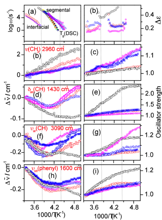
Figure 1: Comparison of inter and intra-molecular dynamics of polyphenylmethylsiloxane in 1- and 2-D dimensional confinement: (a) inter molecular segmental dynamics from BDS; bulk (filled squares), confined in nanoporous silica of pores sizes: -8 nm (circles), 6 nm (triangles) 4 nm (stars). Crossed symbols denote silanized pores. Half filled symbols are dynamics in thin films ranging from 80–7 nm thickness. (b) the corresponding dielectric strength of bulk and confined in pores. (b–i) the temperature dependence of bandshift of the spectral position and oscillator strength of the intra-molecular IR-vibrations in PMPS.
