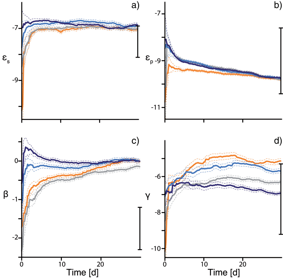
Figure 6. Evolution of four closure parameters (a–d) with assimilation of real observations showing the distribution mean (solid lines) and spread (dashed lines) for different initial parameter distributions (colors). The parameter values are shown in log space, and the vertical black range displays possible parameter values chosen by expert elicitation.
