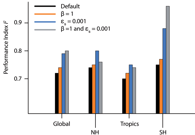
Figure 8. Aggregated error of simulated climate runs, using four different parameter settings. A run with default parameter setting is compared with the runs in which \epsilon_s and \beta are changed individually and simultaneously. Four geographical regions are shown: the global average, the northern hemisphere (NH), southern hemisphere (SH), and the tropics. A low I^2 value corresponds to a good performance. In contrast to the original composition of observables, a reduced set of observations described by Stevens et al. (submitted manuscript, 2012) is used.
