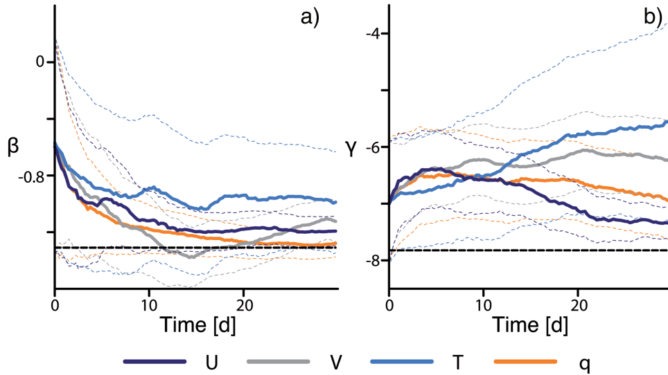
Figure 5. Sensitivity of closure parameters \beta (a) and \gamma (b) to different observation quantities, showing the distribution mean (solid lines) and spread (dashed lines). Parameters are shown in log space, and the dashed black line displays the default parameter value that was set in the run to generate the synthetic observations on a homogeneous observation network. Experiments assimilating only U , V , T , and q are shown in purple, gray, blue, and orange, respectively.
