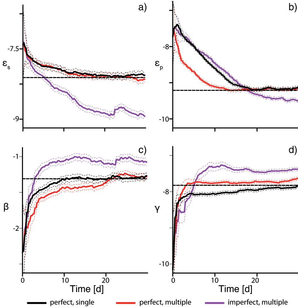
Figure 4. Evolution of four closure parameters (a–d) with different model settings showing the distribution mean (solid lines) and spread (dashed lines). The parameter values are shown in log space, and the dashed black line displays the default parameter value that was set in the run to generate the synthetic observations on a realistic observation network. Three different model setups are displayed: perfect-model results with single parameter estimation (black), four parameters estimated simultaneously (red), and four parameters estimated simultaneously with perturbed gas constant and gravity (purple).
