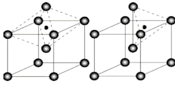
Fig. 1. Positions of an interstitial atom in the bcc structure.
