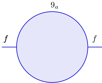
Figure 2: The amplitude \mathcal{D}_{g_a}(f) : a disk whose boundary lies on the D9_a branes, with the insertion of the gauge field at the quadratic order.
