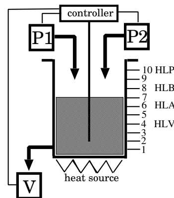
Figure 1. System scheme.
