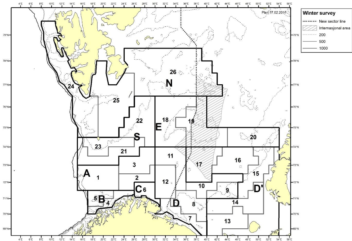
Figure 2.1. Strata (1-23) and Main Areas (A,B,C,D,D',E and S) used for swept area estimations and acoustic estimations with StoX. The Main Areas are also used for acoustic estimations with BEAM. Additional strata (24-26, Main Area N) are covered since 2014, but not included in the full time series.
