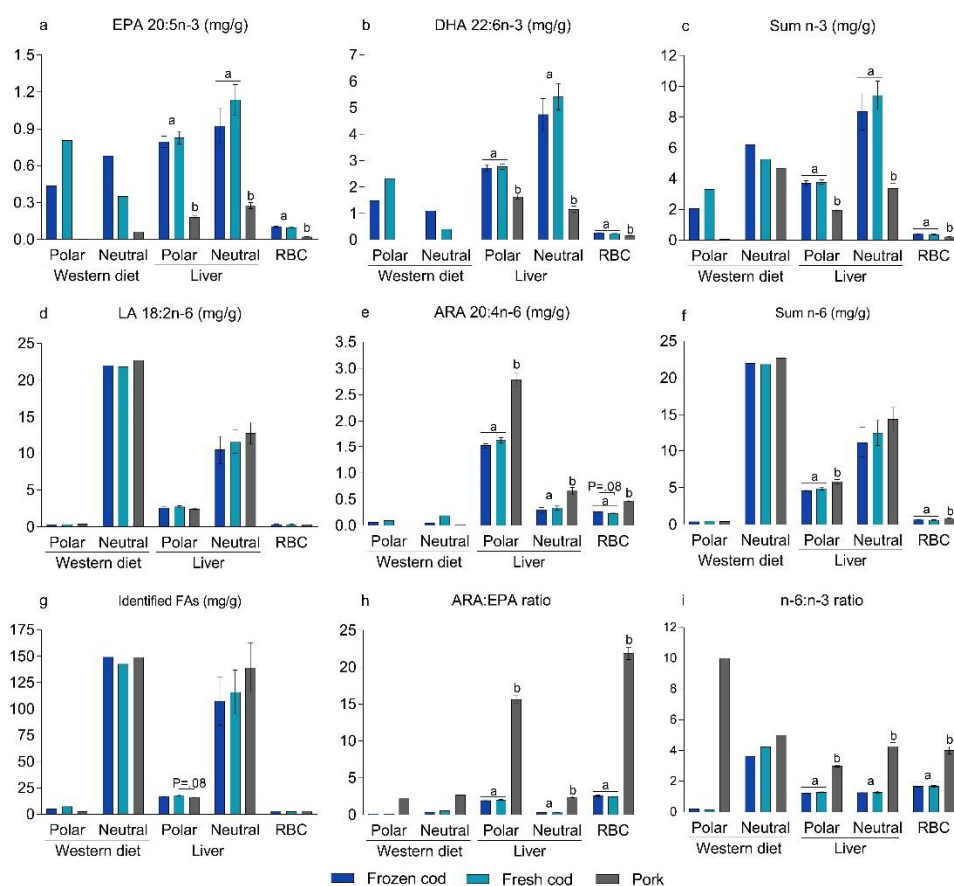
Figure 2. Fatty acid (FA) composition in polar and neutral lipid fractions in Western diets based on frozen cod, fresh cod, and pork as protein sources, and in mouse livers and red blood cells (RBCs) following intake of the different diets. Data from the Western diets represent the means of three samples, and data from the livers and RBCs represent means \pm SEMs ( n = 10 ). Results indicate mg FAs in the polar and neutral lipid fractions/g Western diet and livers, and mg FAs/g RBCs. Lipids from Western diets and livers were extracted and separated into polar and neutral lipid fractions. The FA compositions of the fractions from the Western diets and livers as well as the FA compositions of extracted lipids from RBC were quantification and determined; (a) eicosapentaenoic acid (EPA); (b) docosahexaenoic acid (DHA); (c) sum n-3 ; (d) linoleic acid (LA); (e) arachidonic acid (ARA); (f) sum n-6 ; (g) identified fatty acids (FAs); (h) arachidonic acid: eicosapentaenoic acid ratio (ARA:EPA); (i) n-6:n-3 ratio. Data from livers and RBCs were analyzed using one-way ANOVA followed by Fisher's LSD post hoc tests. Different letters denote statistical significance ( p \leq 0.05 ) between the groups.
