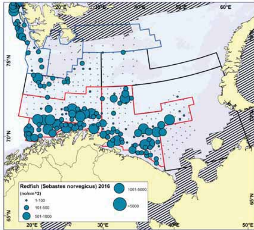
Figure 7.1. Sebastes norvegicus . Distribution in the trawl catches winter 2016 (number per \text{nm}^2 ). Zero catches are indicated by black points.
