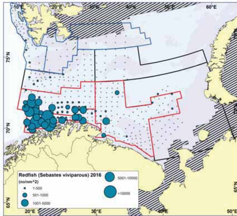
Figure 7.3. Sebastes viviparus . Distribution in the trawl catches winter 2016 (number per nm 2 ). Zero catches are indicated by black points. Species identifications of S. viviparus found north of areas ABCD might be unsure and need verification.
