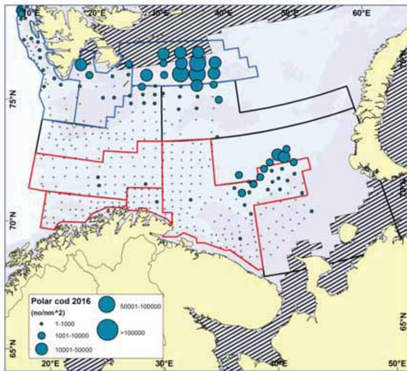
Figure 9.2 POLAR COD. Distribution in the trawl catches winter 2016 (number per \text{nm}^2 ). Zero catches are indicated by black points.
