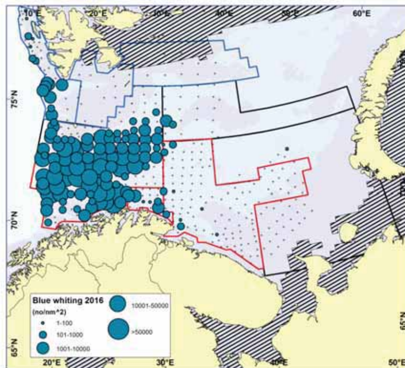
Figure 9.3 BLUE WHITING. Distribution in the trawl catches winter 2016 (number per \text{nm}^2 ). Zero catches are indicated by black points.
