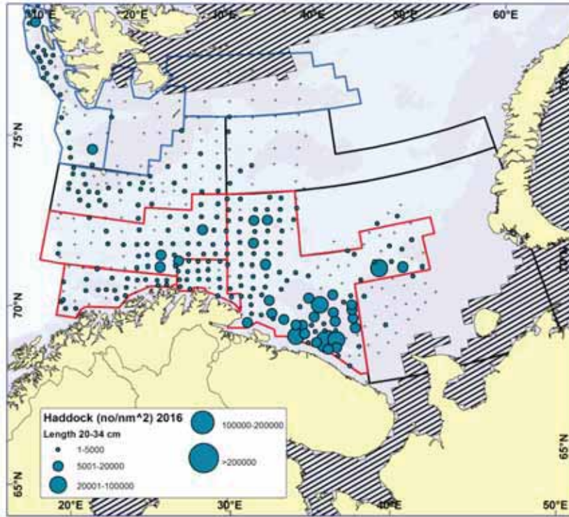
Figure 6.2. HADDOCK 20-34 cm. Distribution in valid bottom trawl catches winter 2016 (number per \text{nm}^2 ). Zero catches are indicated by black points.
