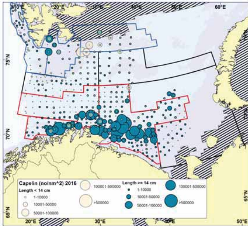
Figure 9.1. CAPELIN. Distribution in the trawl catches winter 2016 (number per \text{nm}^2 ). Zero catches are indicated by black points.
