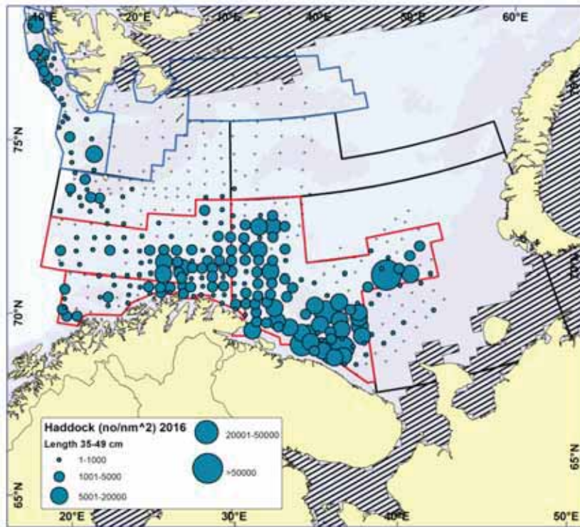
Figure 6.3. HADDOCK 35-49 cm. Distribution in valid bottom trawl catches winter 2016 (number per \text{nm}^2 ). Zero catches are indicated by black points.
