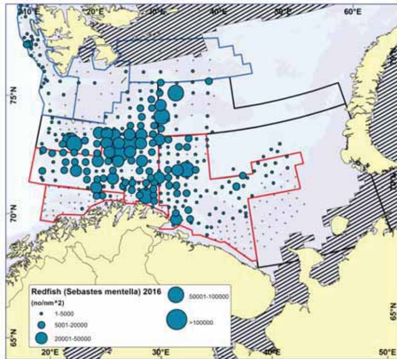
Figure 7.2. Sebastes mentella . Distribution in the trawl catches winter 2016 (number per \text{nm}^2 ). Zero catches are indicated by black points.
