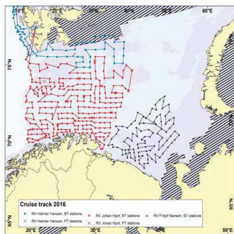
Figure 3.1. Survey tracks and all trawl stations in the winter survey 2016. Data source for the monthly ice cover (hatched areas): ftp://sidads.colorado.edu/DATASETS/NOAA/G02135/shapefiles/
