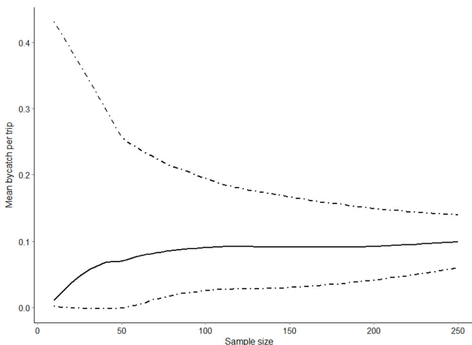
Fig. 2. Trend lines representing the sensitivity of mean bycatch-per-trip estimates (y-axis), as a function of sample size, i.e., number of trips sampled (x-axis). Solid line represent the median bycatch rate, upper dotdashed line represent the 95% percentile and lower dotdashed line the 5% percentile of the estimated bycatch rate. Each sample size was randomly drawn with 500 iterations from a data set representing bycatch data from the cod gillnet fishery of the Reference fleet in 2009 ( n = 455 ).
