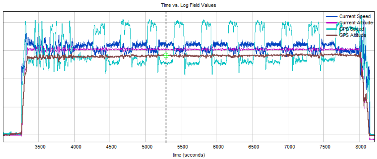
Figure 9. Altitude, airspeed and groundspeed from autopilot airpressure and GPS sensors. From the CW1 flight on 22 March.
