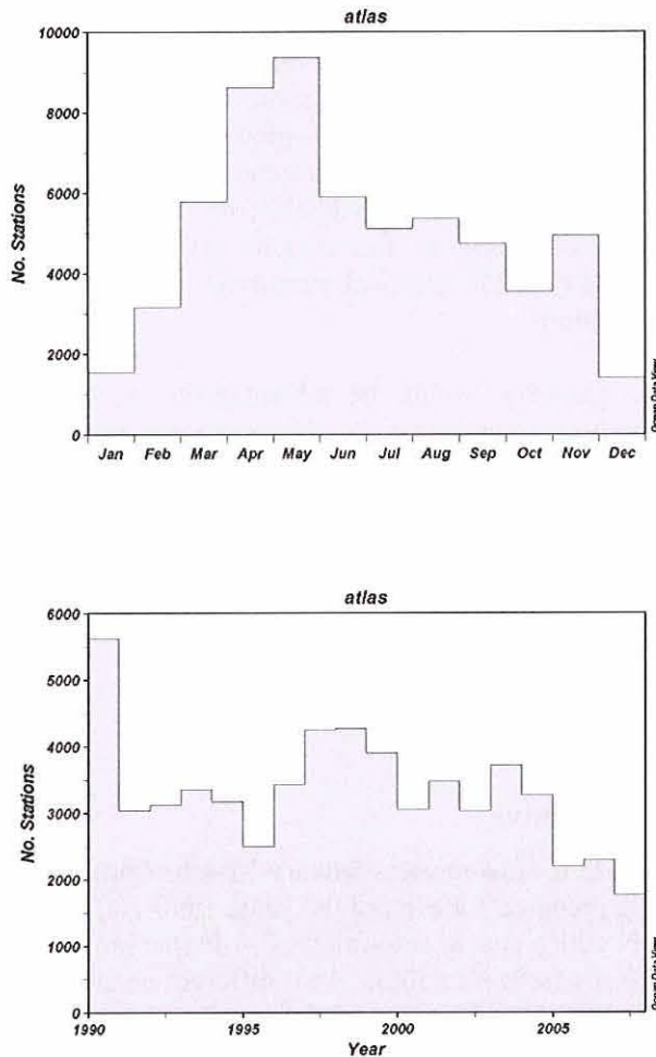
Figure 5. Temporal distribution of stations among months (upper panel) and years (lower panel). Note that while in the upper panel the abbreviation for the month along the x-axis is centred below the corresponding bar, in the lower panel the value for year is positioned to the left of the corresponding bar.
