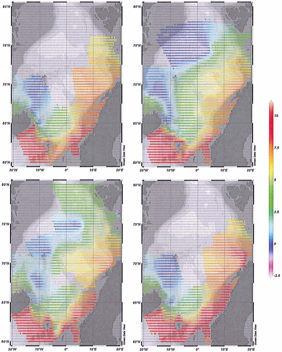
Figure 12. 2D temperature fields at 200 m depth from the temperature atlas based only upon actual data for 2005 per season: Upper left: January-March, upper right: April-June, lower left: July-September, lower right: October-December. Original values for each (non-missing) grid cell shown.
