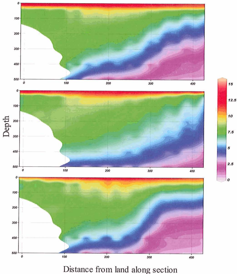
Fig. 21. Example of interannual differences along a vertical profile. The Svinøy section from 62° 22'N, 5° 12'E to 64° 40'N, 0°E at 0-500m depth for the quarter July-September: a) Climatological values for 1990-2007, b) 1990, and c) 2000. Temperature atlas based upon both data and WOA05 climatology used. ODV DIVA interpolation plug-in used for visualization. Moderately non-linear colour scale with higher colour resolution towards lower and higher values applied.
