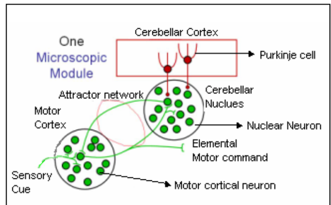
Figure 6. One microscopic module.
