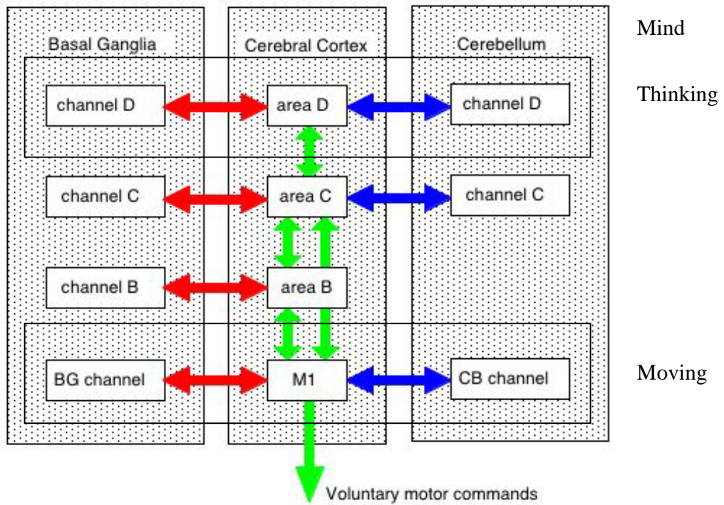
Figure 1. DPMs communicate with each other through cortical-cortical connections.
