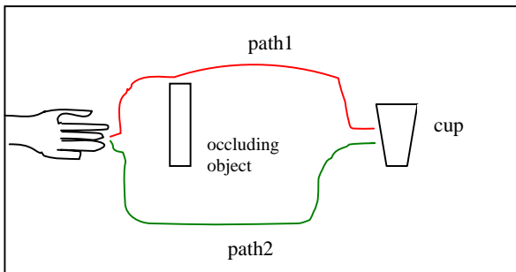
Figure 2. Two possible paths that cerebral cortex selects and sends to basal ganglia for deciding on one.
