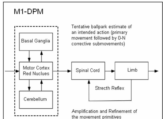
Figure 3. The pattern selection, amplification and refinement process.
