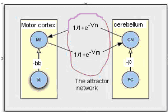
Figure 8. One computational microscopic module.
