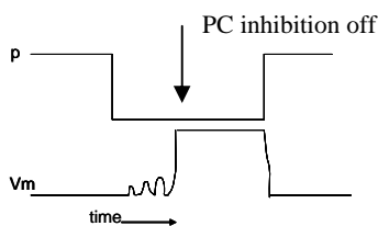
Figure 7. Signaling for a movement command initiation.
