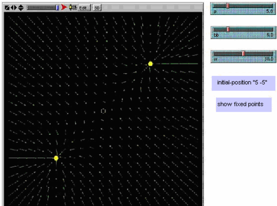
Figure 9. Vector fields and fixed points of an attractor network.
