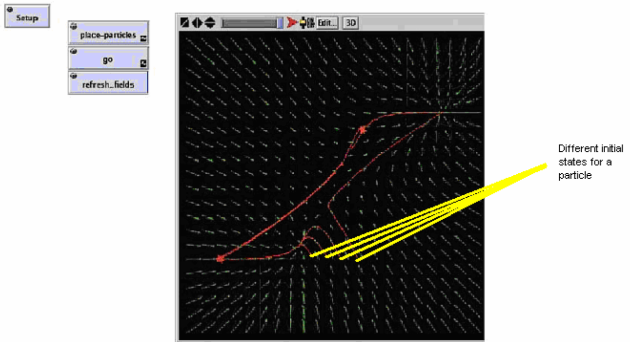
Figure 10. Vector fields and fixed points of an attractor network.
