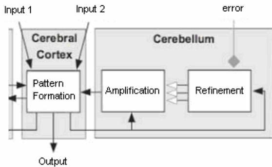
Figure 4. M1 cortical-cerebellar loop.
