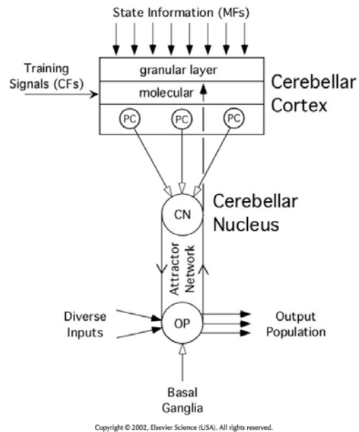
Figure 5. One macroscopic module.
