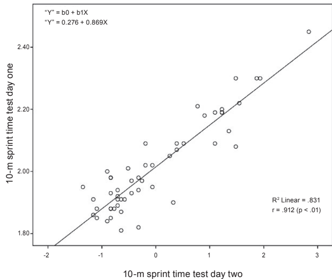
Figure 1. R 2 , Pearson's r correlation coefficient, p -value and linear regression equation between the results of the 10-m sprint time test day one and 10-m sprint time test day two.
