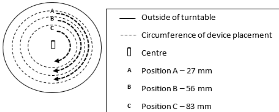
Figure 5. Turntable schematic
