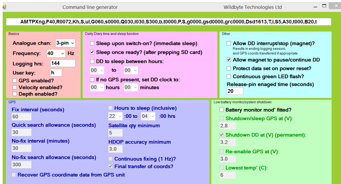
Figure 18. Command line generator for SlamTracker device
