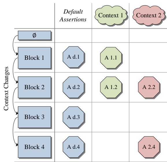
Figure 2: Concept of block-based context-sensitive testing
