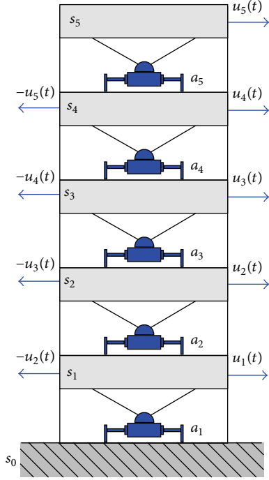
FIGURE 1: Five-story building actuation scheme.
