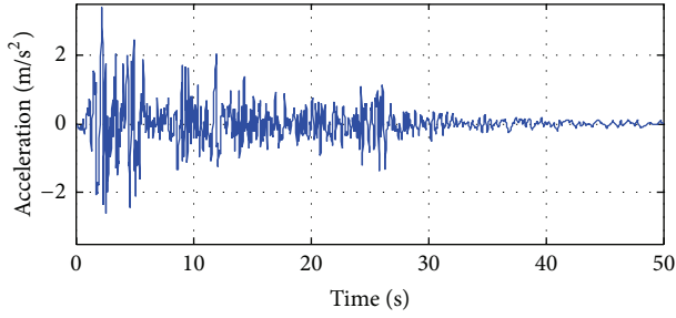
FIGURE 2: Full scale North-South El Centro 1940 seismic record.
