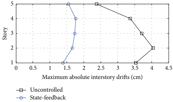
FIGURE 3: Maximum absolute interstory drifts corresponding to the uncontrolled building (black line with rectangles) and the controlled building with the ideal state-feedback energy-to-peak controller defined by the gain matrix \tilde{G}_s (blue line with circles). The full scale North-South El Centro 1940 seismic record has been used as ground acceleration disturbance.
