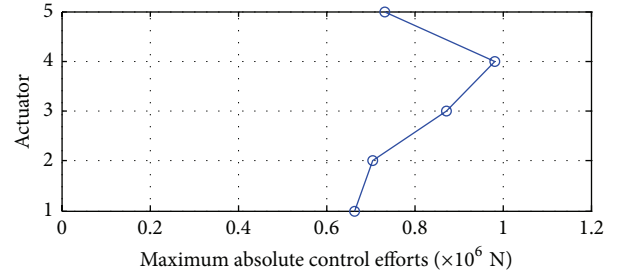
FIGURE 4: Maximum absolute control efforts corresponding to the controlled building with the ideal state-feedback energy-to-peak controller defined by the gain matrix \tilde{G}_s . The full scale North-South El Centro 1940 seismic record has been used as ground acceleration disturbance.
