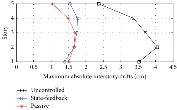
FIGURE 5: Maximum absolute interstory drifts corresponding to the uncontrolled building (black line with rectangles), the ideal state-feedback energy-to-peak controller defined by the gain matrix \tilde{G}_s (blue line with circles), and the passive-damping system defined by the gain matrix \tilde{K}_d (red line with asterisks). The full scale North-South El Centro 1940 seismic record has been used as ground acceleration disturbance.
