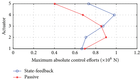
FIGURE 6: Maximum absolute control efforts corresponding to the ideal state-feedback energy-to-peak controller defined by the gain matrix \tilde{G}_s (blue line with circles) and the passive-damping system defined by the gain matrix \tilde{K}_d (red line with asterisks). The full scale North-South El Centro 1940 seismic record has been used as ground acceleration disturbance.
