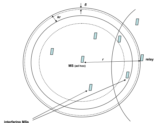
Fig. 2. Basic Model for Total Interference Calculation (Ad Hoc to Relay).
