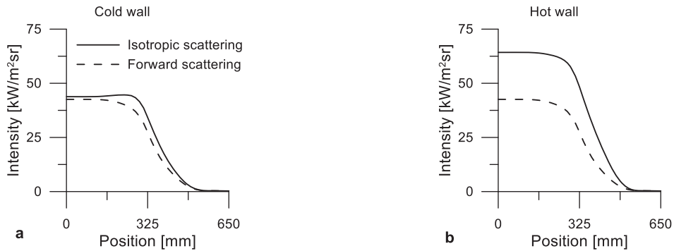
Figure 17. Full isotropic scattering of the incoming radiation is compared to forward-scattering for a flame with a solid fuel. The wall temperature is 500°C (a) or 1200°C (b).
