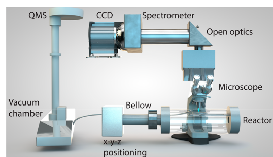
Figure 1. Overview of the setup that is centered on a flow-reactor tube made from glass. To enable dark-field scattering spectroscopy, the reactor tube is equipped with a flat 200 \mu\text{m} thick optical window. The flow reactor arrangement is mounted on the sample stage of an upright optical microscope. It is connected to a spectrometer equipped with a CCD camera to collect scattered light from (individual) catalyst nanostructures via a long-working-distance 50 \times dark-field objective and epi-illumination. It is also equipped with a gas inlet connected to mass-flow controllers for accurate control of reactant concentration and reactant flow. The quadrupole mass spectrometer (QMS) is mounted on a high-vacuum chamber that is connected to the flow reactor chamber via a stainless steel tube. To enable the QMS readout directly from the close vicinity of the nanofabricated sample surface, we use a glass capillary “sniffer” mounted inside the flow reactor. It acts as orifice leak and has a \sim 5 \mu\text{m} opening. Its position can be accurately controlled via an x-y-z micrometer stage. To control sample temperature, the system is internally equipped with a flat ceramic carbon heater that serves as the sample holder for the nanofabricated model catalyst.
