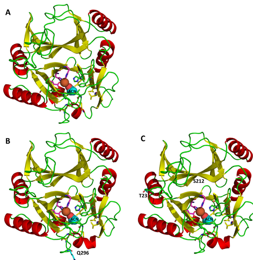
Figure 1. The deduced 3-D structure of the wild type (A) and mutant forms: C230B65 (B) and C230B81 (C) of C230 from Planococcus sp. S5.
