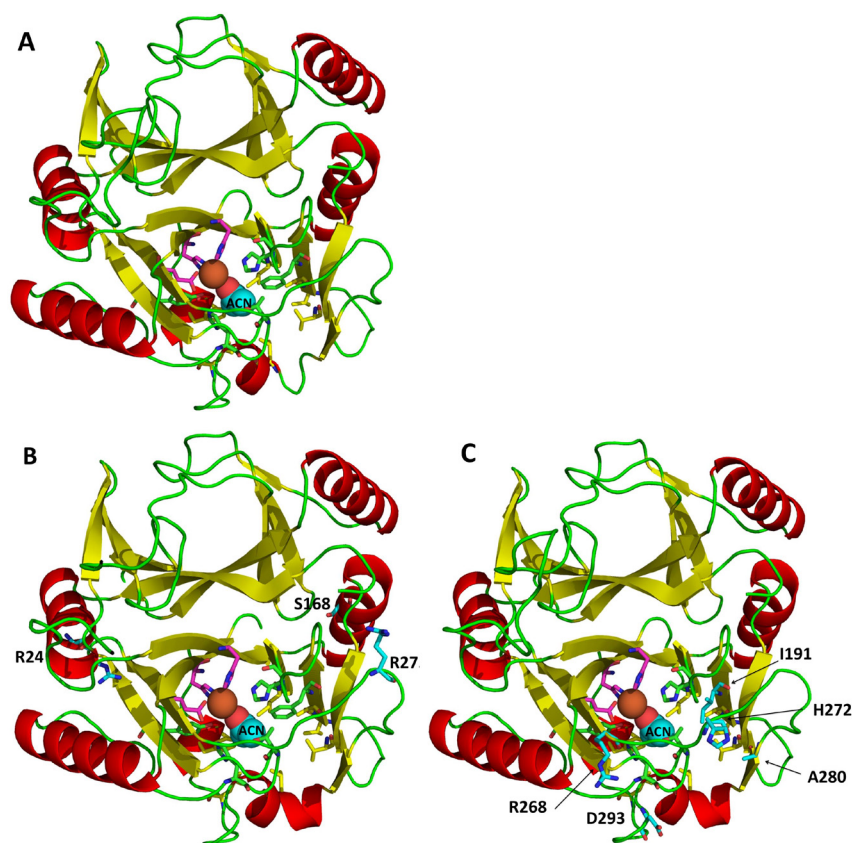
Figure 2. The deduced 3-D structure of the wild type (A) and the mutant forms: C23OB58 (B) and C23OC61 (C) of C230 from Planococcus sp. S5.
