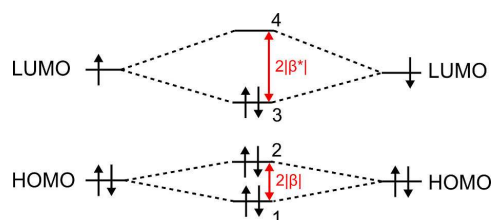
Scheme 1. Orbital correlation diagram from TCNQ anion-radicals to (\text{TCNQ})_2^{2-} showing the dimer level splitting 2|\beta| and 2|\beta^*| for the HOMO- and LUMO-derived dimer orbitals, respectively. LUMO becomes SOMO when it is singly occupied. Orbital No 3 is the bonding combination of the two SOMO orbitals. [11]
