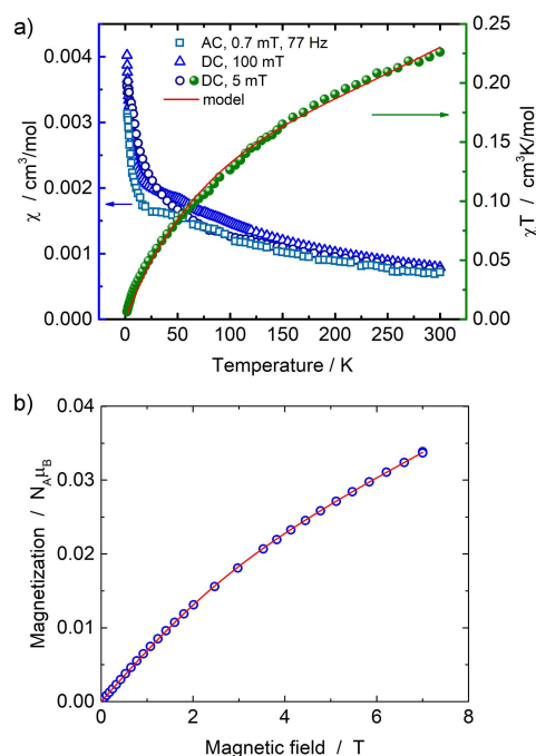
Figure 4. Temperature dependence of magnetic susceptibility (DC mode in fields 5 and 100 mT, AC with 0.7 mT field amplitude) and \chi T product (DC in field 5 mT), including a fit using the model described in the text (a). Field dependence of magnetization of RAS 1 measured at 2 K (b). The model assumes paramagnetic contribution and weak contribution of correlated spins.
