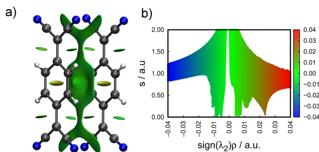
Figure 2. \pi - \pi -interactions in (\text{TCNQ})_2^{\bullet-} dimer, truncated from the crystal structure of 1 . Visualization of intermolecular noncovalent interactions (NCI) between neighboring monomers marked with green color (a). The depicted NCI surface corresponds to the reduced density gradient of 0.5 a.u. NCI plot: the relationship between reduced density gradient ( s ) and the sign of the second eigenvalue ( \lambda_2 ) of the electron density Hessian, as described in [22, 23] (b). Values of the reduced density gradient approaching 0 a.u. in the electron density range of -0.01 < \rho < 0.01 indicate strong inter-radical interactions based on the \pi - \pi stacking, i.e. pancake bonding.
