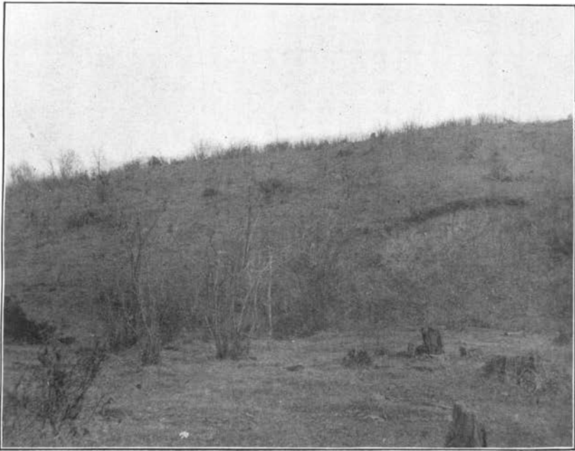
FIG. 1. A gravelly hillside stripped of its forest. Shows beginning of erosion. Algona, Iowa.
