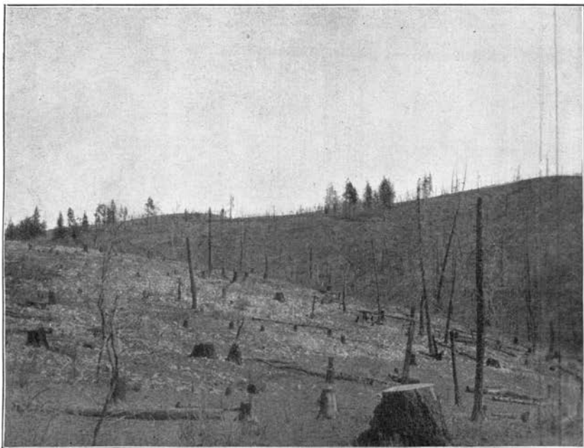
FIG. 1. The cleared mountain slopes. Sacramento mountains, New Mexico. The end.
