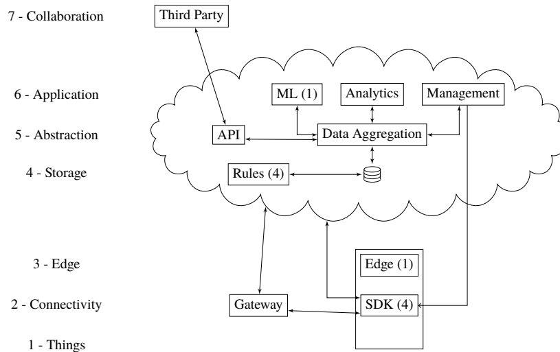
Figure 6.5: “Telecoms” architecture (5 platforms) and the components shared by some (number in brackets) or all (no number) of the platforms
