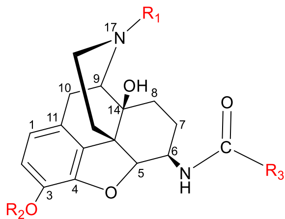
4,5-epoxymorphinan skeleton
