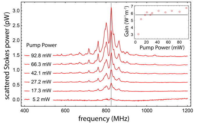
FIG. 5. Spontaneous forward Brillouin Stokes power spectra vs intrafiber pump power. Power spectra are offset 0.3 pW with increasing power for clarity. Inset: estimated Brillouin gain obtained for peak located at 827 MHz (see vertical line). Horizontal line is given by best fit to data, yielding G_B = 5.8 \pm 1 \text{ (W m)}^{-1} .
