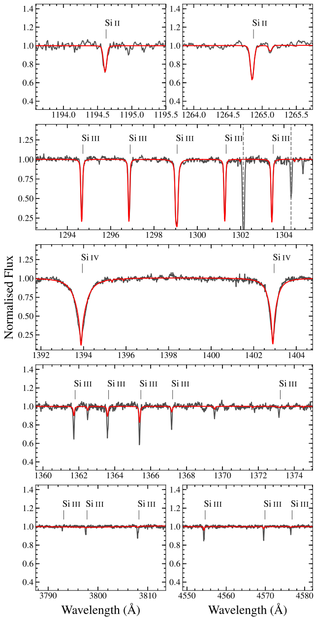
Figure 7. Model atmosphere (red) to various ionization levels of Si. Si II, Si IV, and low-excitation states of Si III (top three panels) are all consistent with an abundance of Si/H \approx -5.9 . Si III lines with excitation energies \gtrsim 7 eV instead require Si/H \approx -5.1 in both the STIS and HIRES spectra (bottom two panels).
