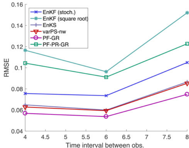
Fig. 14. RMSE as a function of the time interval between observations for a partially observed KdV system.
