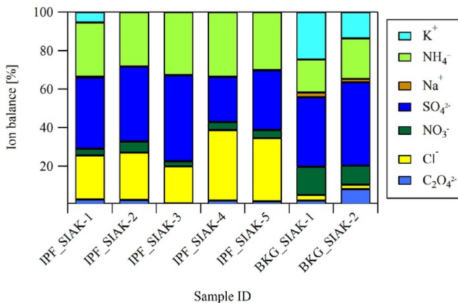
Fig. 2. Percentage of anion and cation contribution to total PM_{2.5} ions based on equivalent concentrations at Indonesian peatland fire (IPF) and background (BKG) sources in Siak (SIAK).
