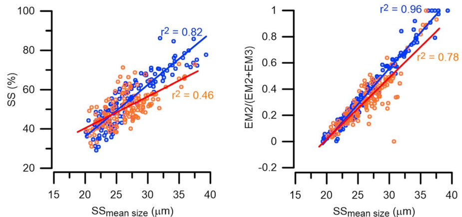
Figure 7. (a) Cross plot of the mean sortable silt (SS) fraction (10–63 μm) and the percentage of silt within the fraction <63 μm of core 905 (blue circles) and core 909 (orange circles). (b) Cross plot of the SS mean and the ratio between EM2/(EM2 + EM3). EM = end-member.
