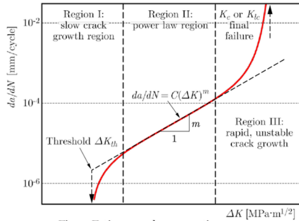
Fig. 7. Fatigue crack propagation curve
