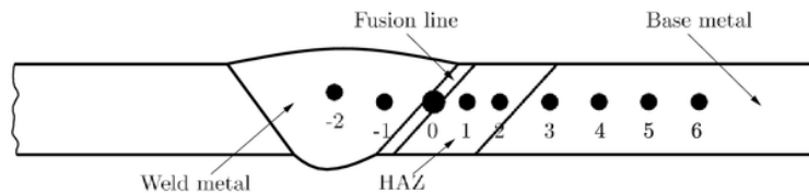
Fig. 2. Welding profiles and a schematic illustration of the hardness testing distribution
