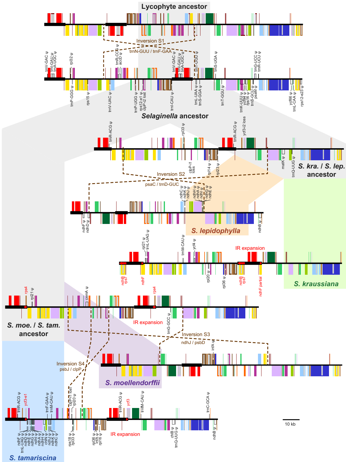
Fig. 3 Structural evolution of Selaginella plastomes. Pseudogenes and lost genes are marked with a \psi and listed in black text. Inversion endpoints are marked by brown dotted lines, and the genes closest to each endpoint are listed in brown text. Inverted repeat (IR) expansions are denoted with red arrows, and genes affected by the IR expansion are listed in red text.
