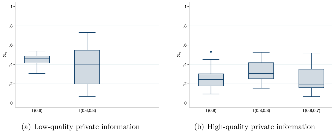
Figure 5: Gini coefficient.
