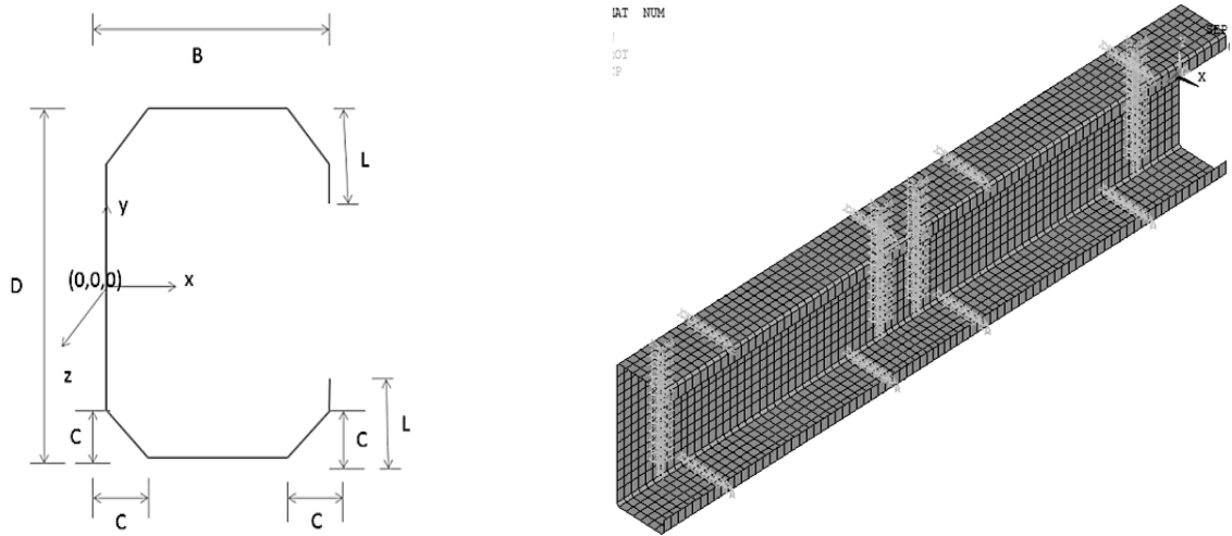
(a) Cross section of the C-section used for the FE model
