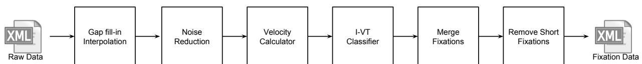
Figure 4. Raw data processing [48].
