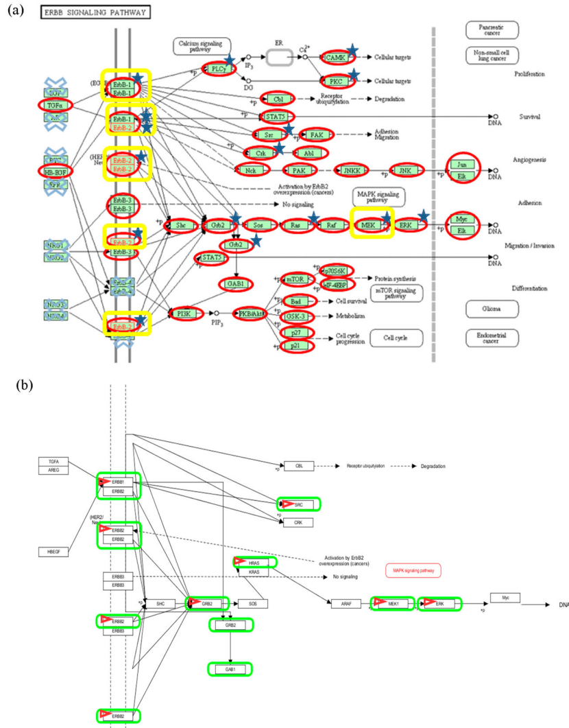
Figure 7. ERBB signaling pathway analysis. (a) Summation of the RNA-Seq and proteomic values for genes present in the ERBB signaling pathway from KEGG. 34 Red circle: RNA-Seq > 1 cutoff value. (The red box means the RPKM value is higher than the cut off. The red color is selected only for better clarity. Note this is a different format for visual clarity as the red circles provide best contrast with the green boxes used in the KEGG figures.) Blue cross = RNA-Seq < 1. Blue star = proteomics spectral count value > 0. Yellow box = proteomics spectral count value > 3 only in ERBB2+ tumor sample. (b) Simplified ERBB signaling pathway that lists only the subpathways with a high number of protein observations (ERBB2+ vs ERBB2- patient samples). All genes illustrated have RPKM value > 1, green box: spectral counts \geq 1; the red star: higher spectral counts in ERBB2+ set (also spectral counts in tumor is higher than control). Note that color is selected only for visual clarity.
