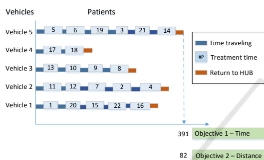
Figure 3: Non-dominated solution that minimizes distance.
