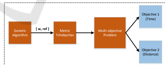
Figure 1: Multi-objective optimization framework.
