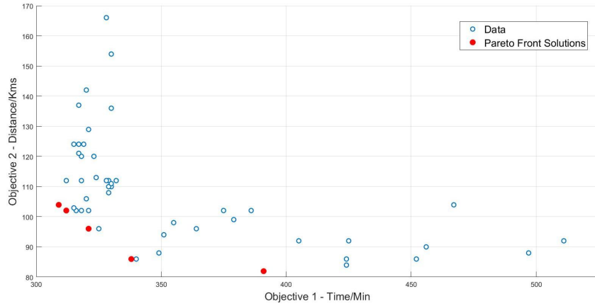
Figure 2: Pareto front and dominated solutions.
