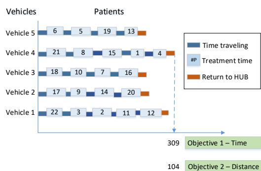
Figure 4: Non-dominated solution that best represents the objective of minimizing time.
