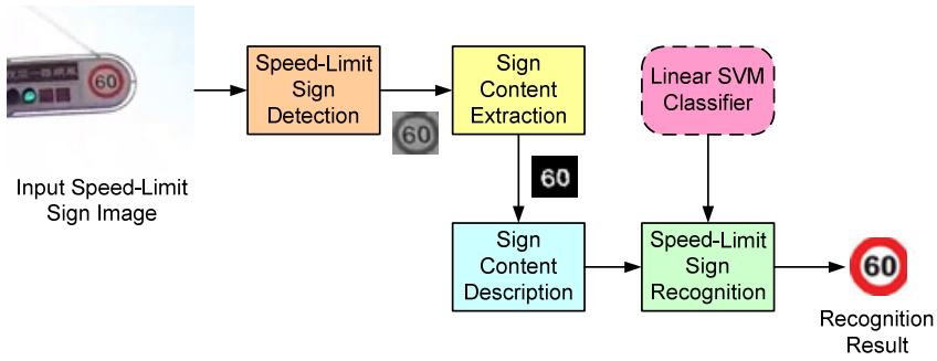
Fig. 1 Block diagram of the proposed SLS detection and recognition system.
