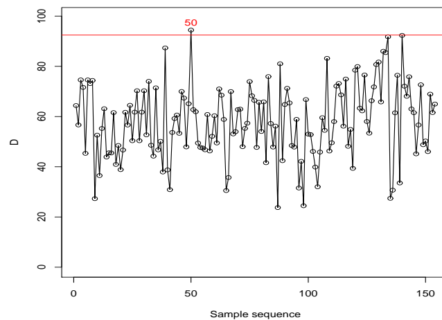
FIGURE 3. The SIGMA-chart for 153 vent-open profiles
