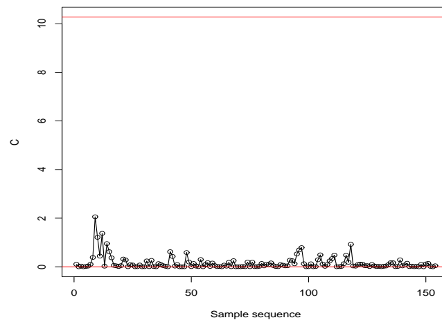
FIGURE 2. The BETA-chart for 153 vent-open profiles
