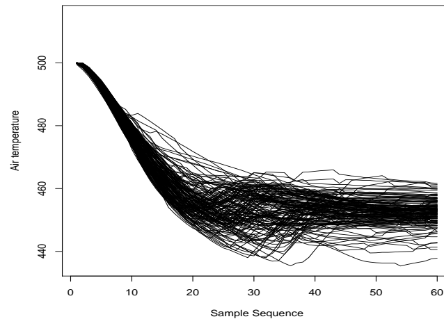
FIGURE 1. 153 in-control profiles in the vent-open stage
