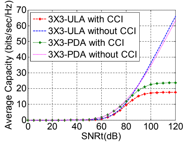
Fig. 5. The average capacities of WLAN systems for both MIMO-ULA and MIMO-PDA with and without single CCI
