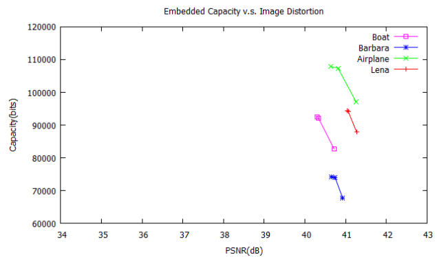
Figure 6. Capacity v.s. image distortion in four test images of embedding watermarks into H_{1,2} subimages.
