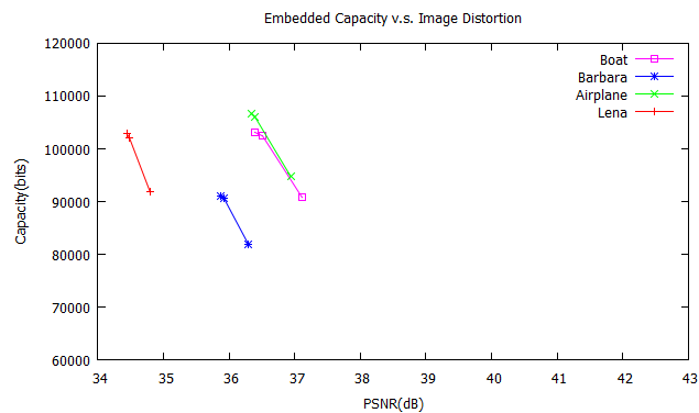
Figure 7. Capacity v.s. image distortion in four test images of embedding watermarks into H_{i,3} subimages.
