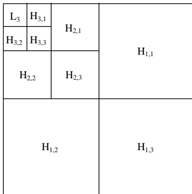
Figure 1. Subimages under integer wavelet transform.
