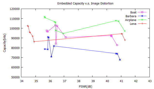
Figure 4. Capacity v.s. image distortion in four test images.
