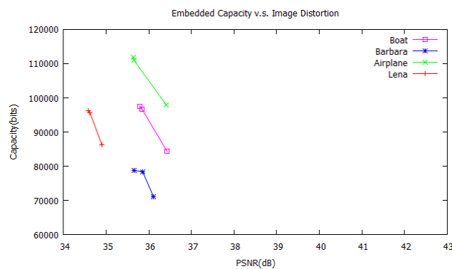
Figure 5. Capacity v.s. image distortion in four test images of embedding watermarks into H_{1,i} subimages.
