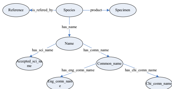
Fig. 5. RDF graph for query 4
