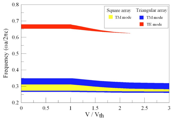
FIG. 9. (Color online) Calculated photonic band gap as a function of normalized voltage. The applied electric field is in the small voltage region. The radius of cylinders is taken as r=0.2a . The colored areas represent tunable band gaps.
