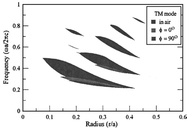
FIG. 3. (Color online) Gap maps for a square lattice of dielectric cylinders.
